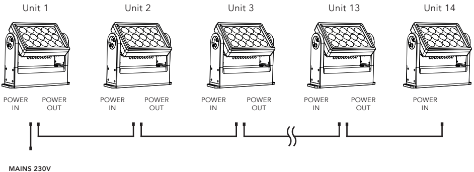
Fig. 05 - Example configuration (Output at 230 V)
