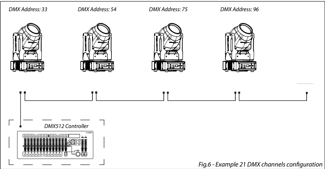
Fig.6 - Example 21 DMX channels configuration
